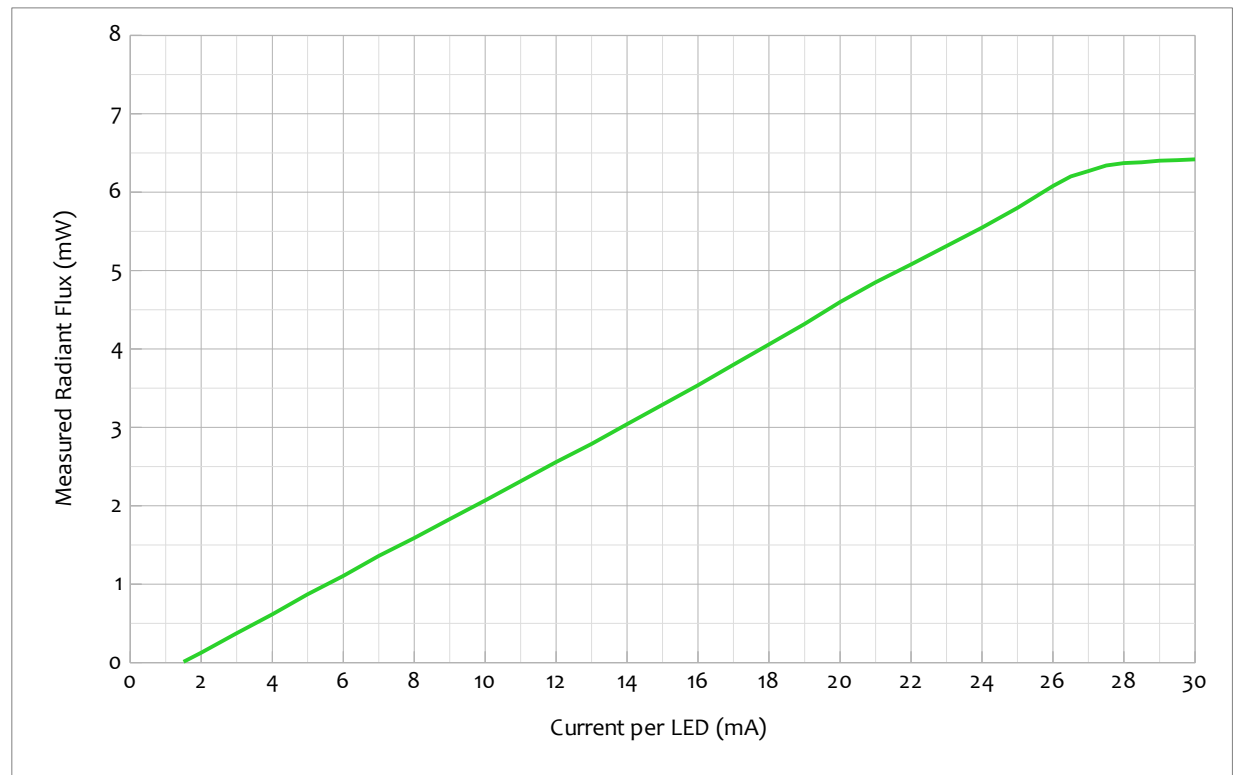
Measured Radiant Flux vs. Current per LED
