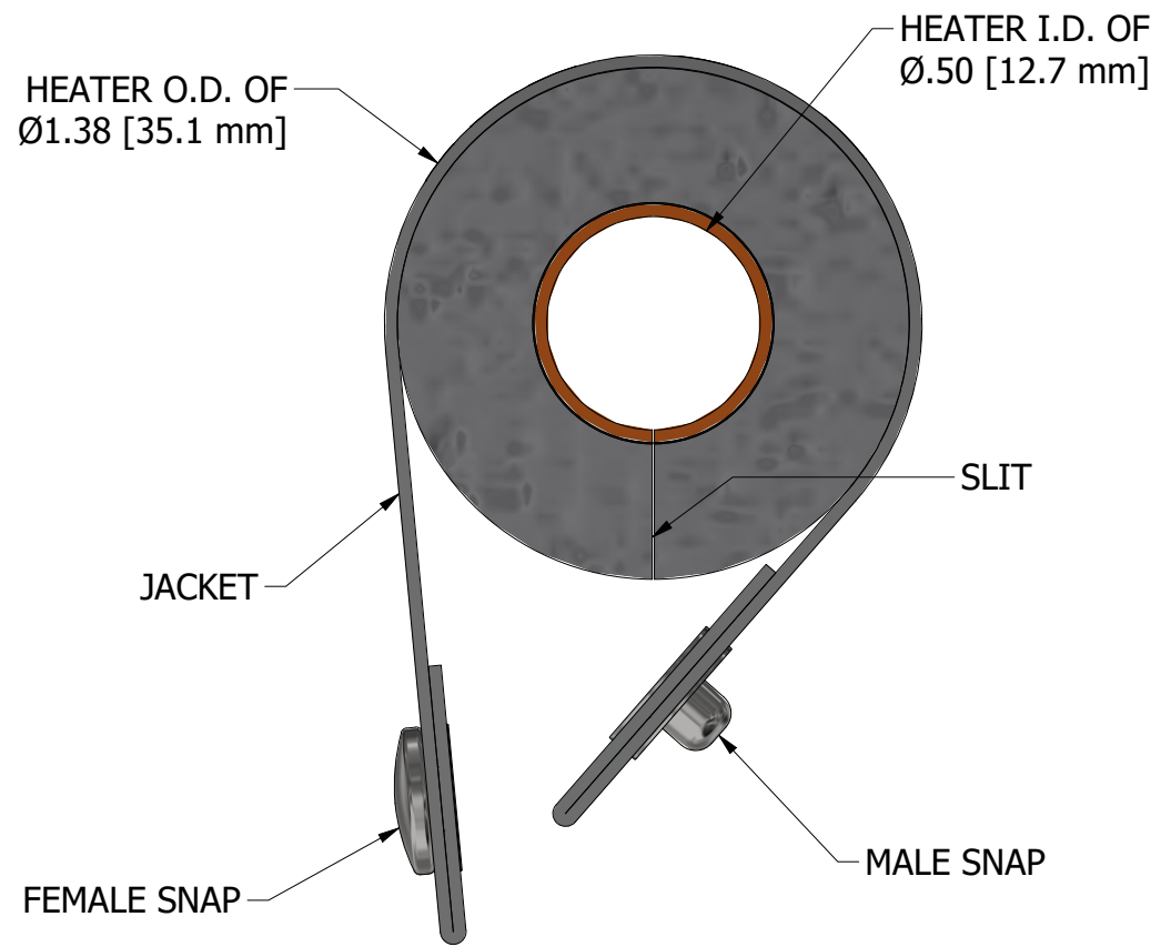
END VIEW SCALE 2 : 1
