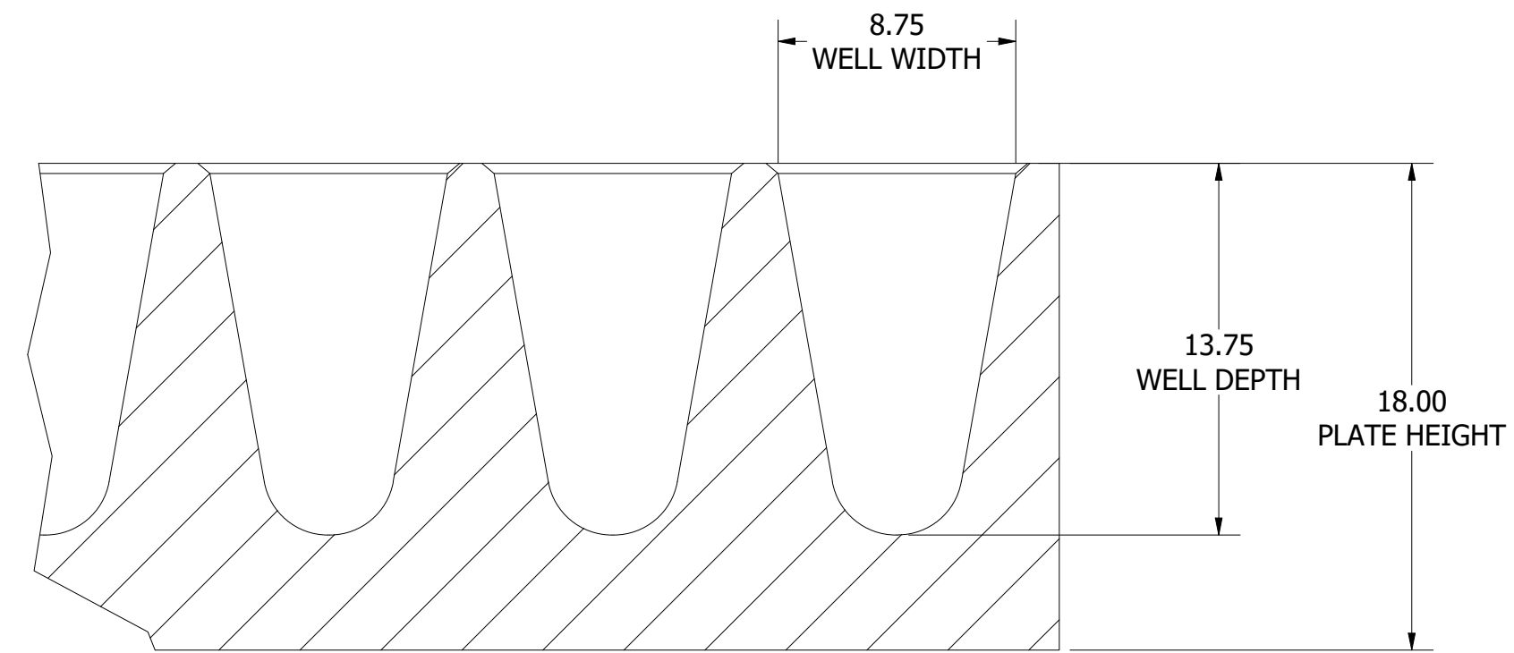
DETAIL B SCALE 4 : 1
