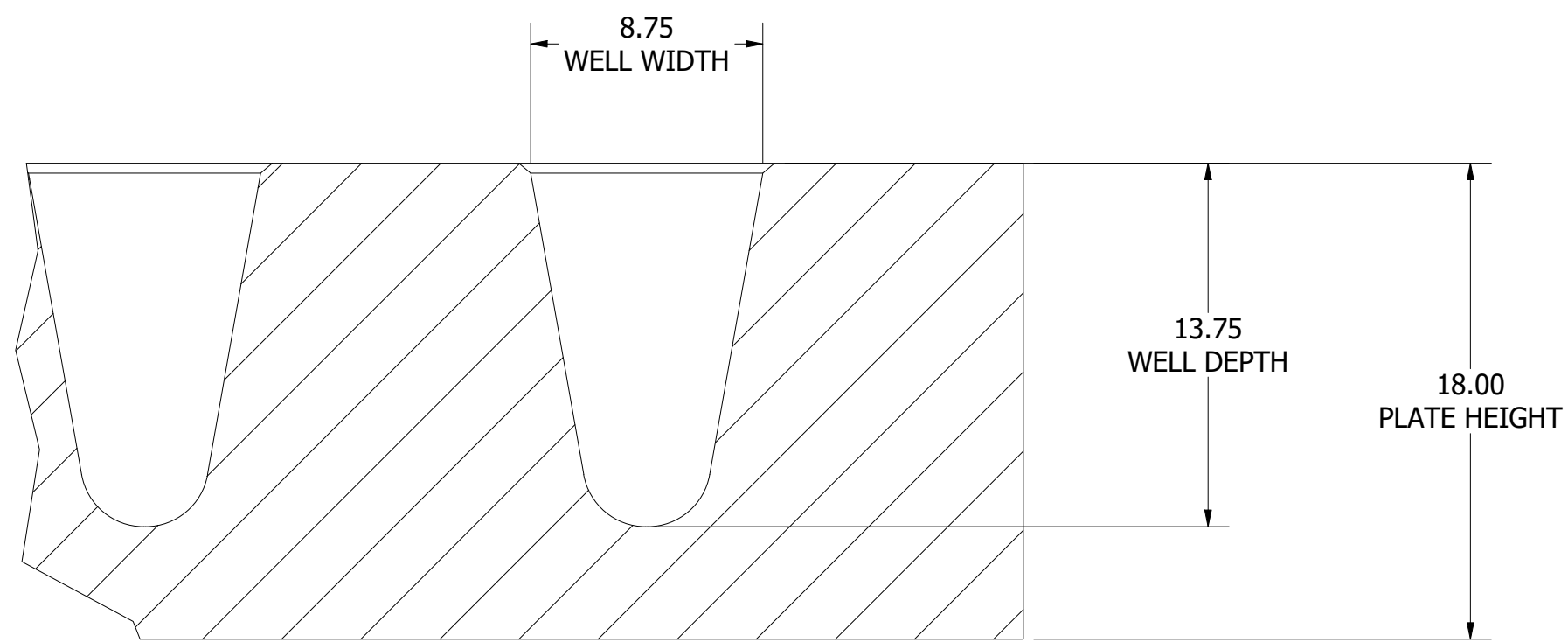
DETAIL B SCALE 4 : 1
