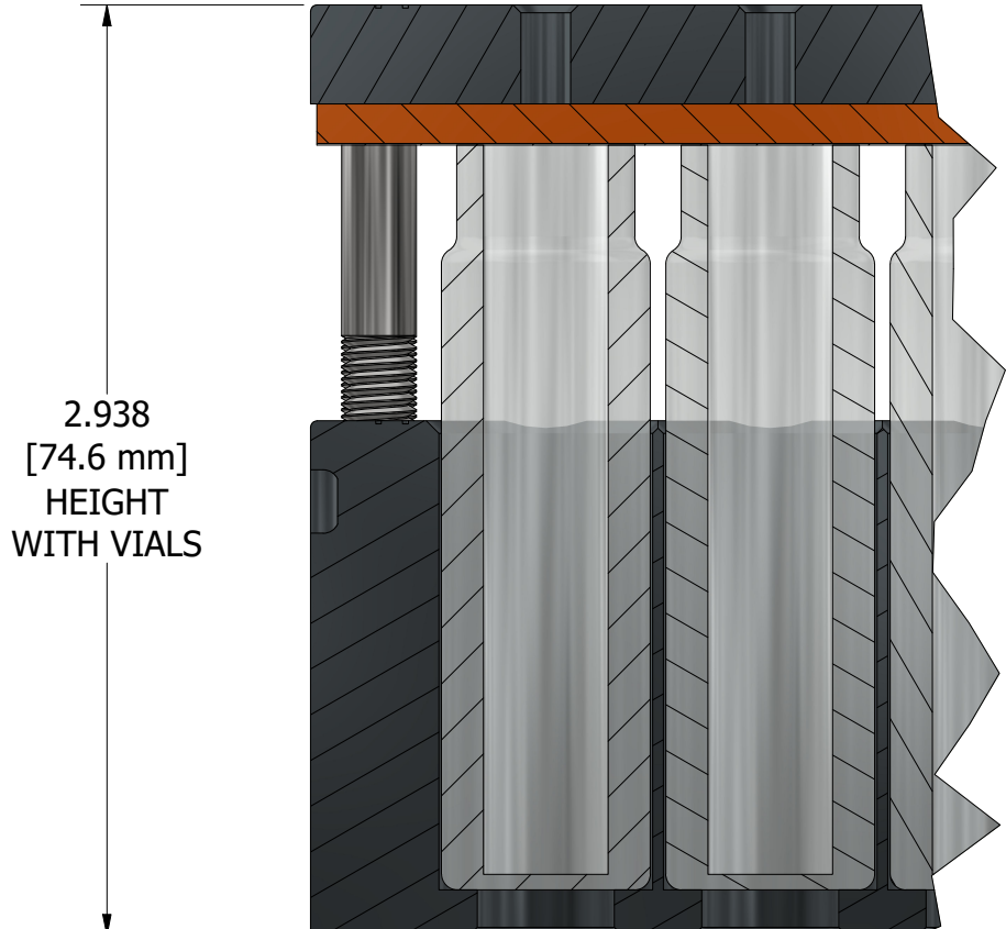
DETAIL A SCALE 3 : 2
