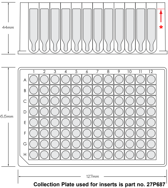
Collection Plate used for inserts is part no. 27P687
