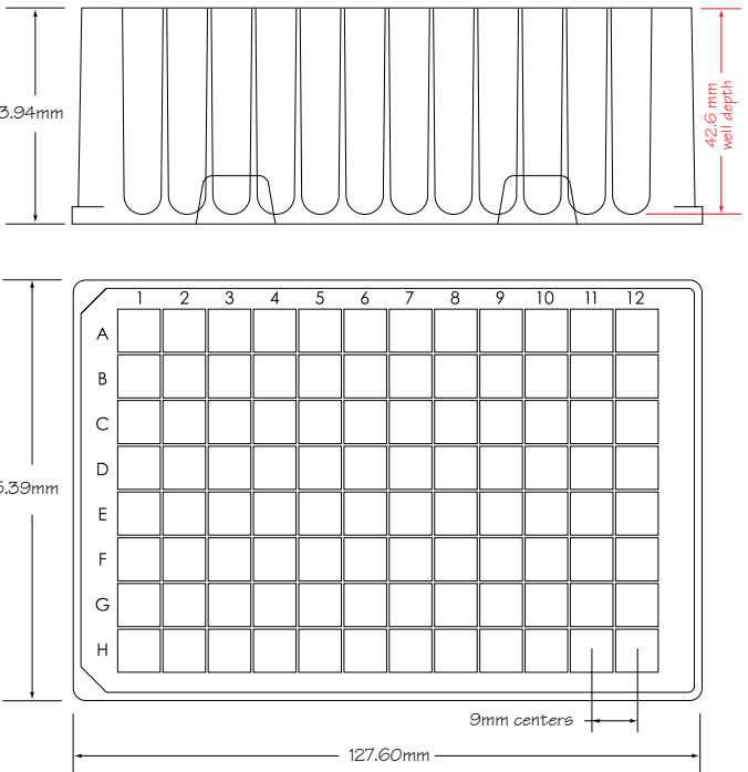
Advantage™ Clear-Vu™ 2mL 96-Well Collection Plates Square Well with Round Bottom
