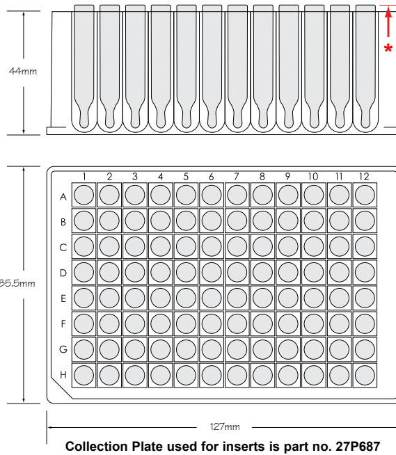
Collection Plate used for inserts is part no. 27P687
