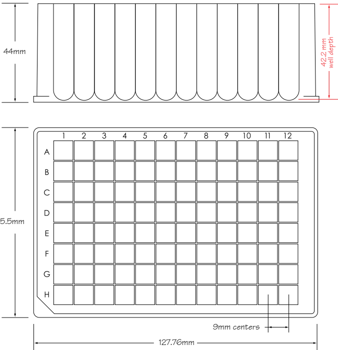
Advantage™ 2mL Polypropylene 96-Well Collection Plates Square Well with Round Bottom
